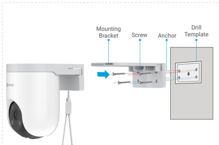
Fig. 2 Wall Mount
