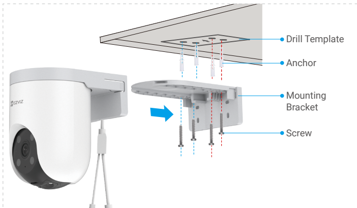
Fig. 1 Ceiling Mount
